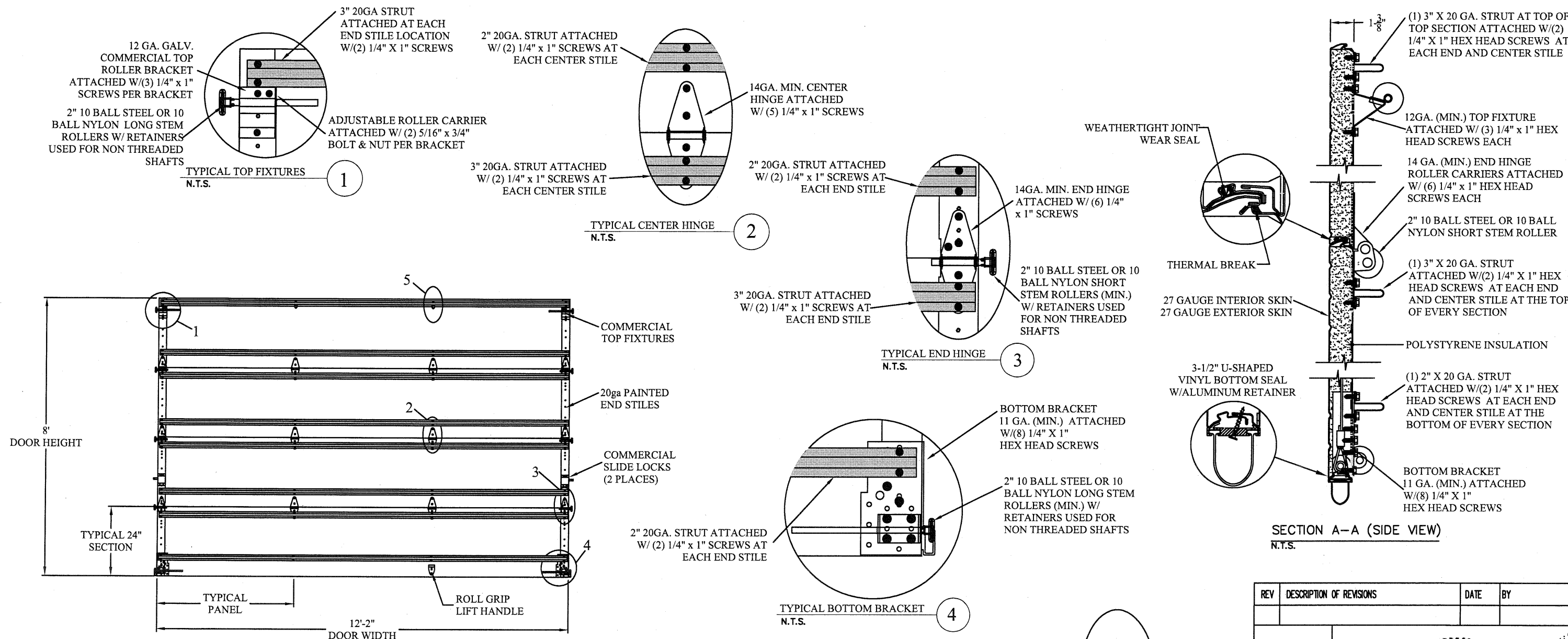
DOOR INTERIOR ELEVATION
